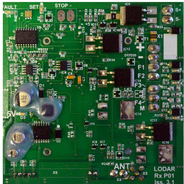
Component Side
