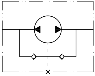
Hydraulic Schematic
