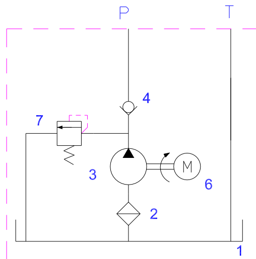
Hydraulic Schematic
